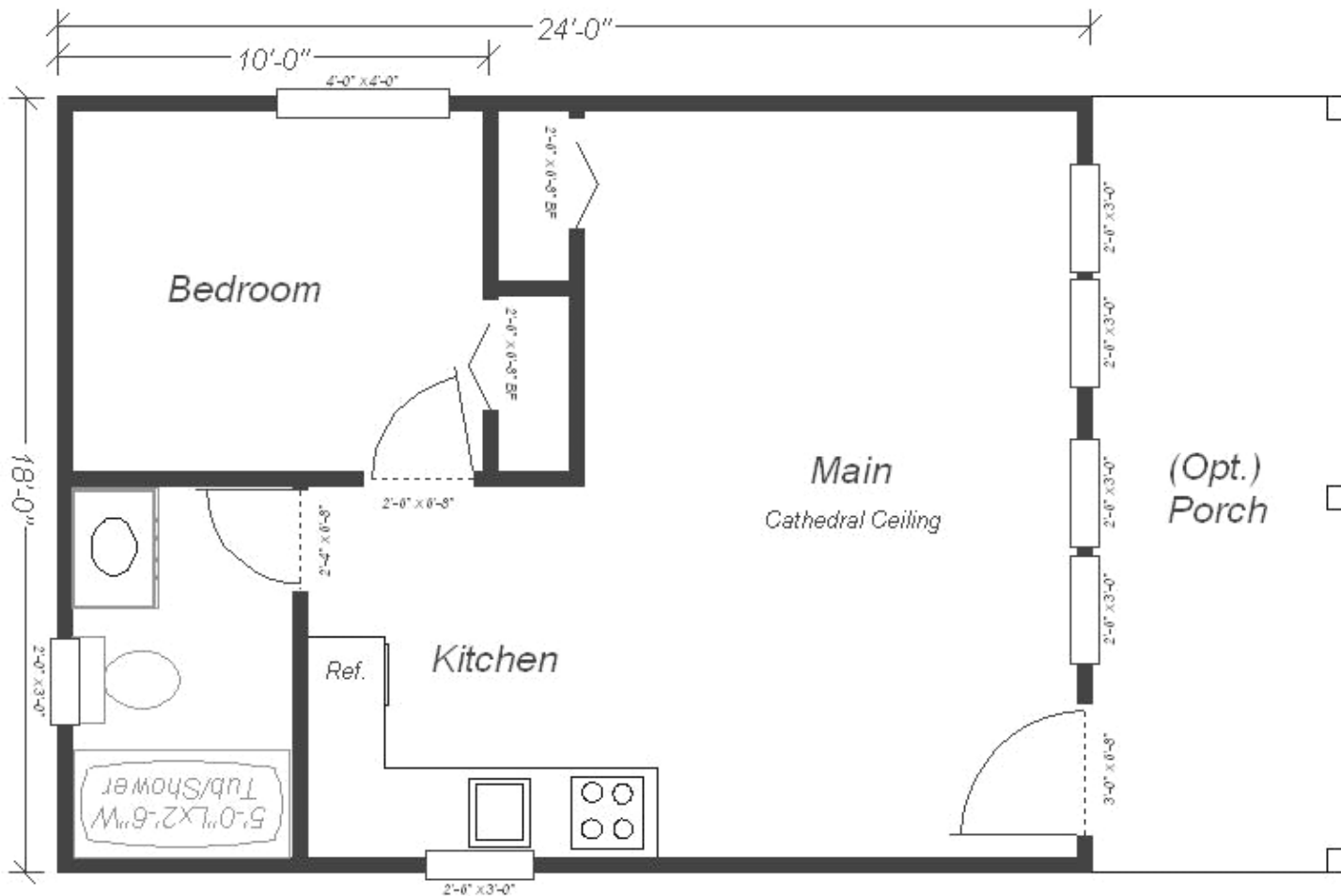
18' x 24' Guest House (432sq.ft.)
