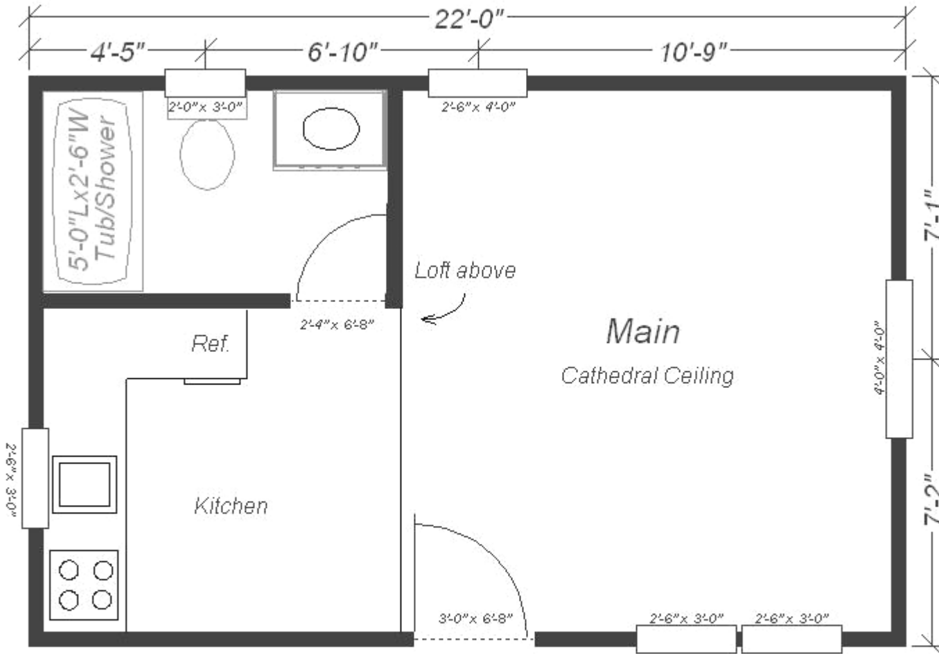
14' x 22' Guest House (308sq.ft.)
